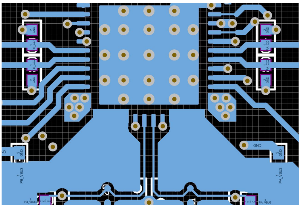
Figure 11-6. VBUS1 and VBUS2 Copper Pours and Via Placement (Top)
