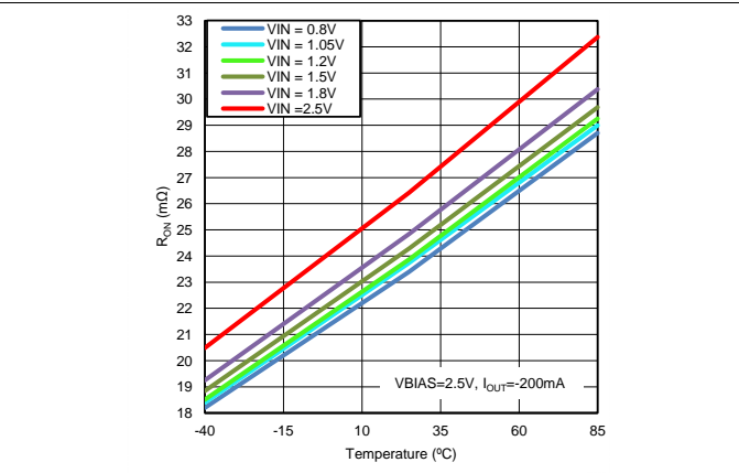
Figure 5. Temperature vs R_{ON} ( V_{BIAS} = 2.5\text{ V} )
