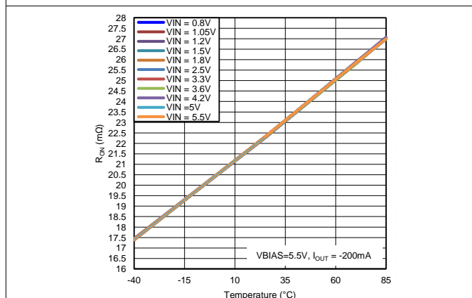
Figure 6. Temperature vs R_{ON} ( V_{BIAS} = 5.5\text{ V} )
