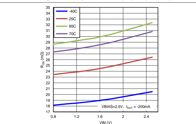
Figure 7. V_{IN} vs R_{ON} ( V_{BIAS} = 2.5\text{ V} )
